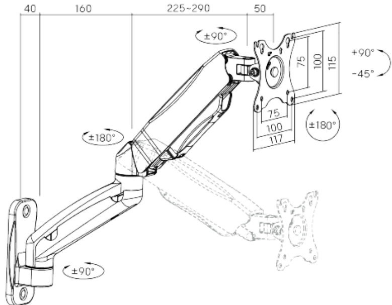
Dimensions (mm)
