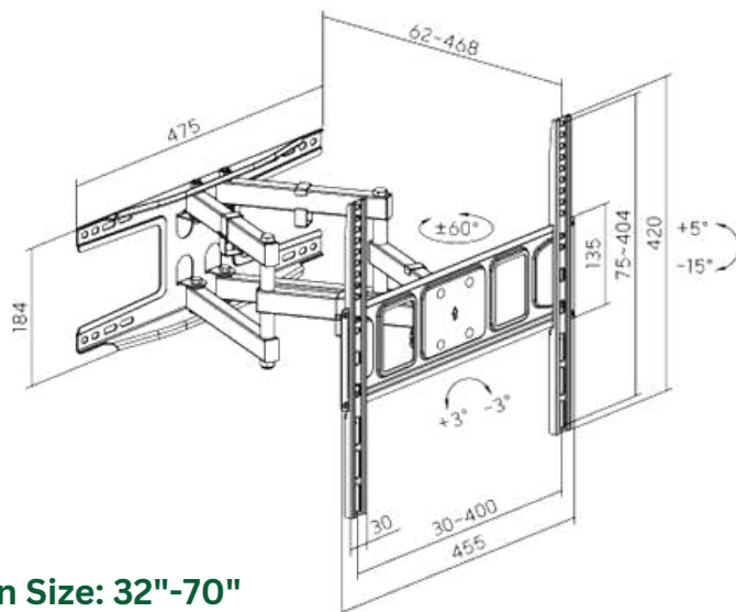
Dimensions (mm)
