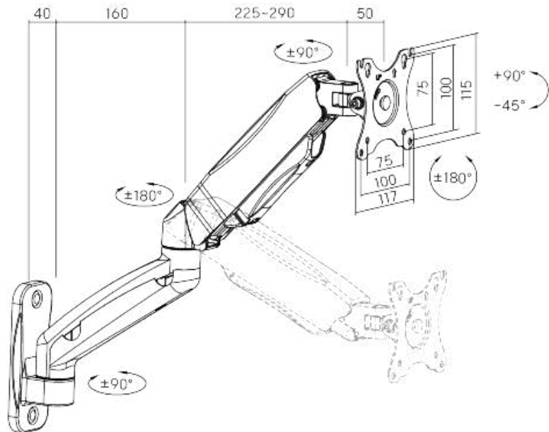
Dimensions (mm)
