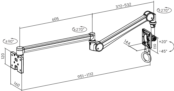
Dimensions (mm)
