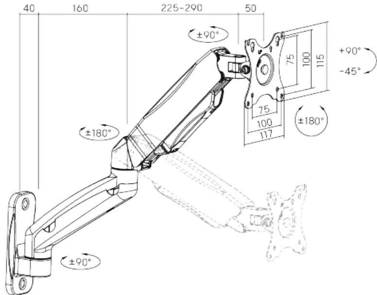
Dimensions (mm)
