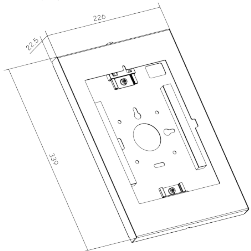
Dimensions (mm)
